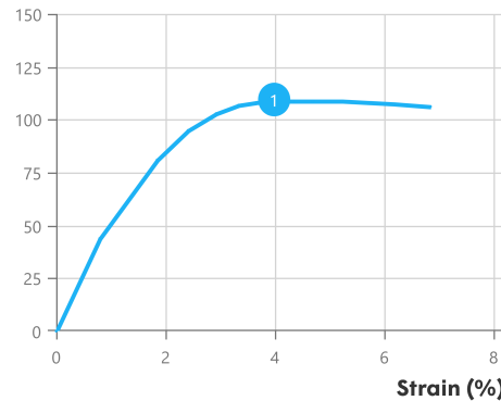
Stress-strain, conditioned
