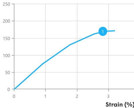
Stress-strain, dry
